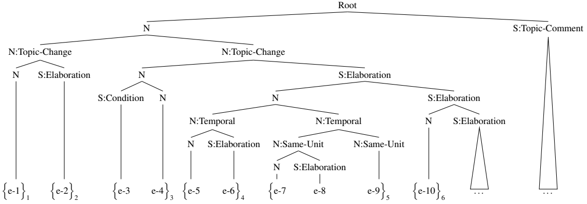
Figure 1: Part of discourse tree (wsj-0623) in RST-DTB: ‘S’, ‘N’ and ‘e’ stand for Satellite, Nucleus and EDU. Each EDU is labeled with its index in the text, and EDUs grouped with {} brackets are in the same sentence.
